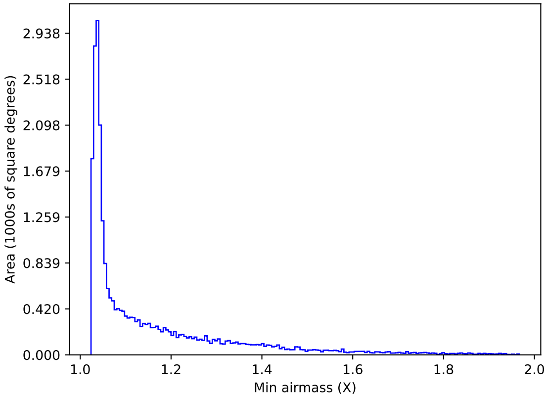
noroll_mjdp60_v3.4_10yrs All sky g band: Min airmass
