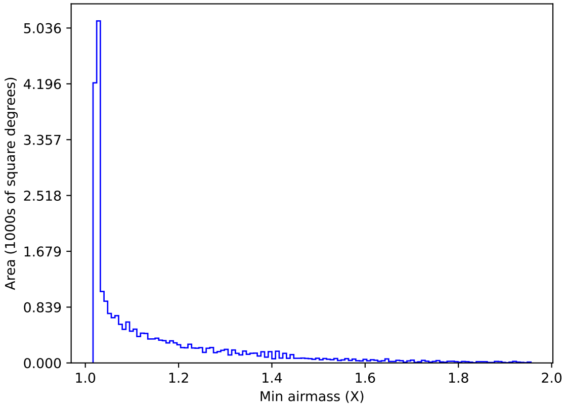
noroll_mjdp60_v3.4_10yrs All sky all bands: Min airmass
