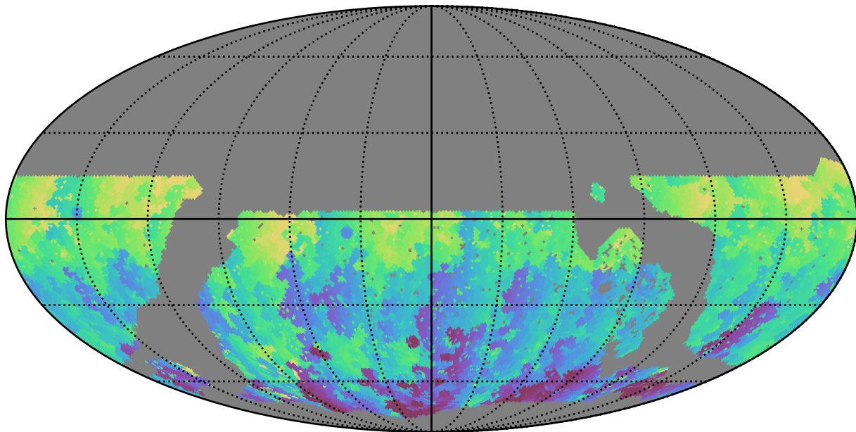
noroll_mjdp60_v3.4_10yrs WFD u band: Min HA
