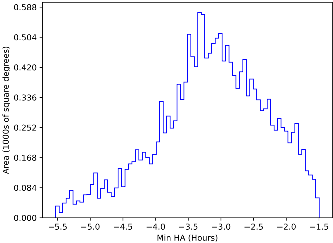
noroll_mjdp60_v3.4_10yrs WFD u band: Min HA
