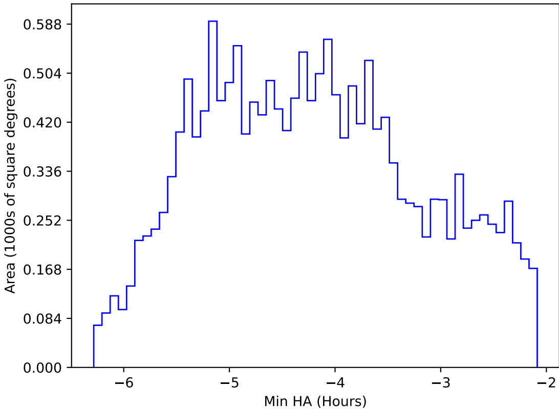
noroll_mjdp60_v3.4_10yrs WFD r band: Min HA
