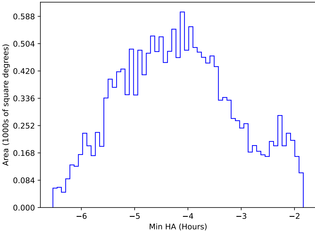
noroll_mjdp60_v3.4_10yrs WFD i band: Min HA
