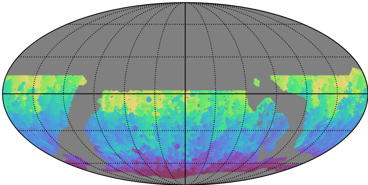
noroll_mjdp60_v3.4_10yrs WFD g band: Min HA
