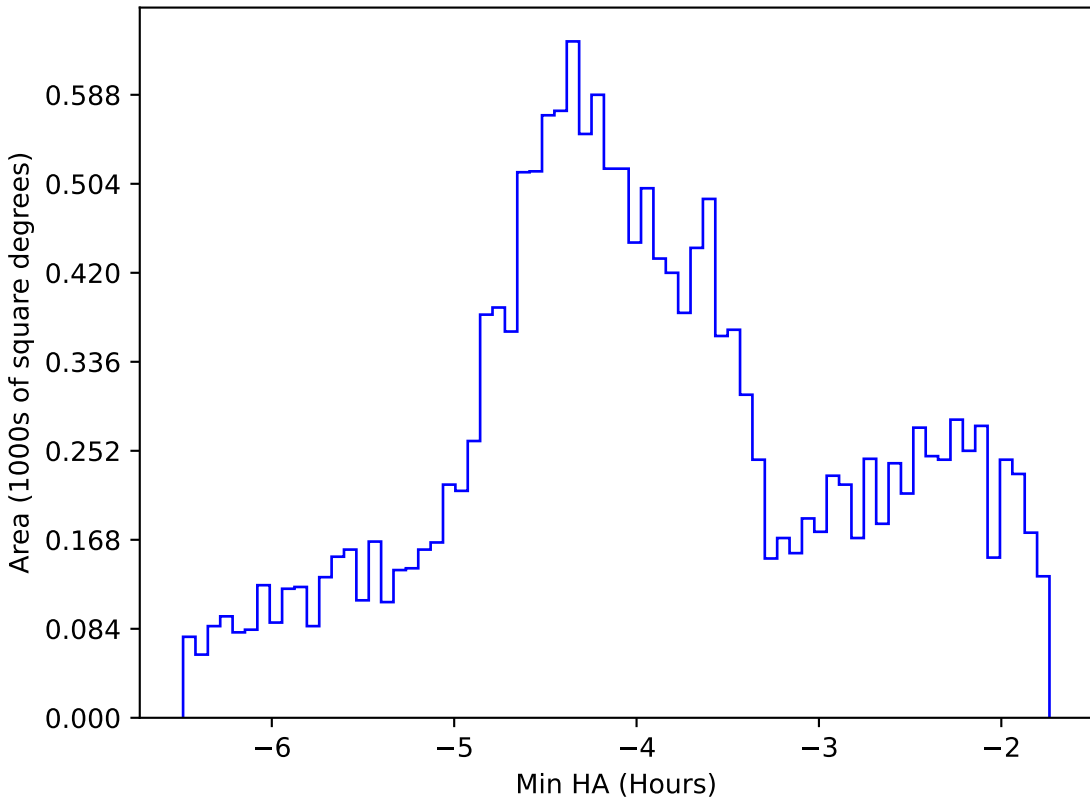
noroll_mjdp60_v3.4_10yrs WFD g band: Min HA
