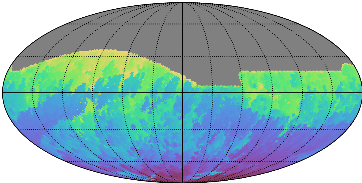
noroll_mjdp60_v3.4_10yrs All sky z band: Min HA
