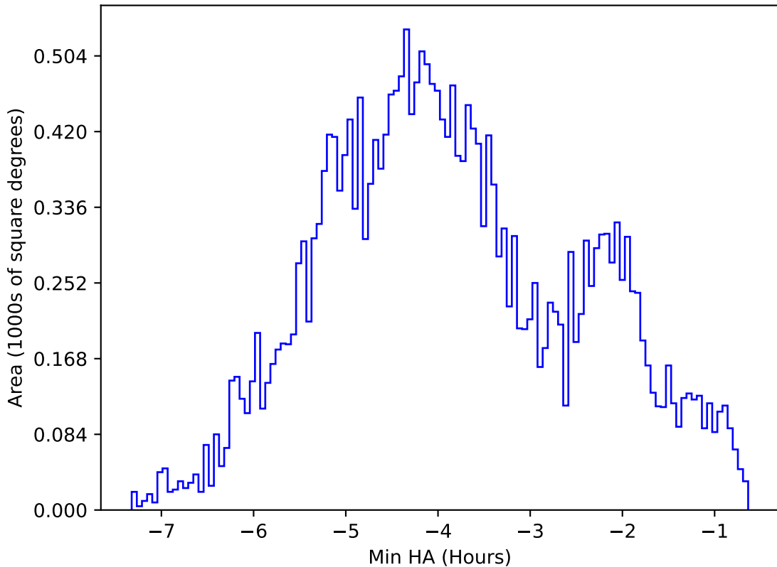
noroll_mjdp60_v3.4_10yrs All sky z band: Min HA
