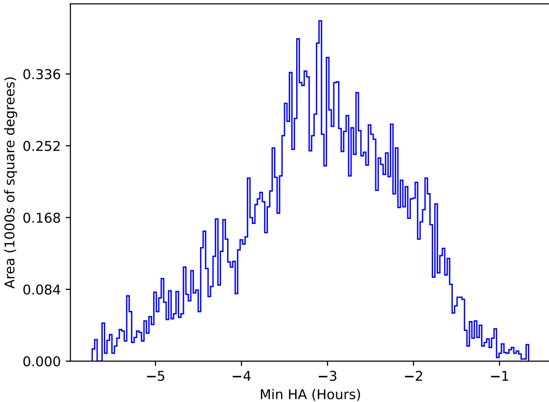
noroll_mjdp60_v3.4_10yrs All sky u band: Min HA
