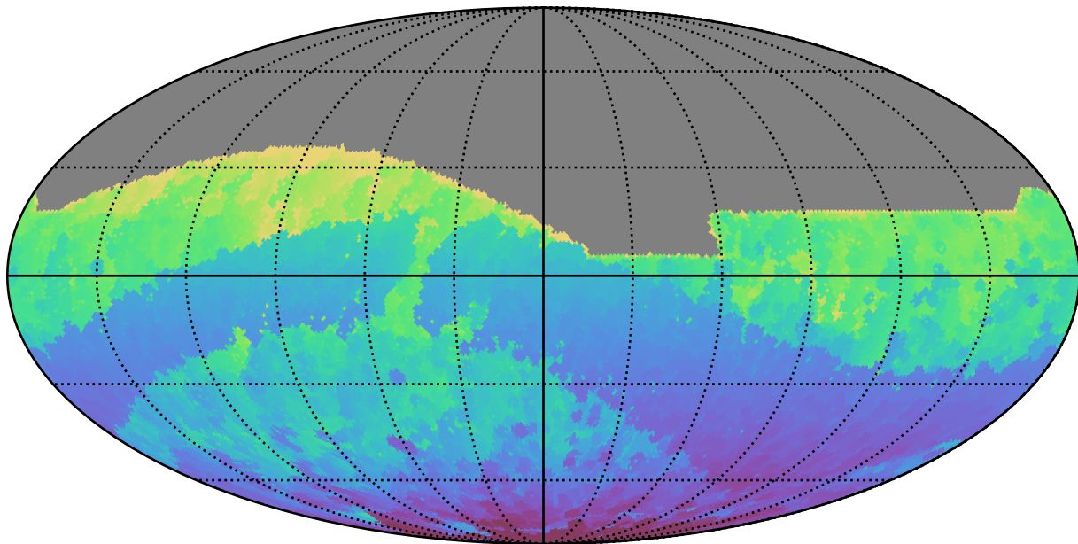
noroll_mjdp60_v3.4_10yrs All sky r band: Min HA
