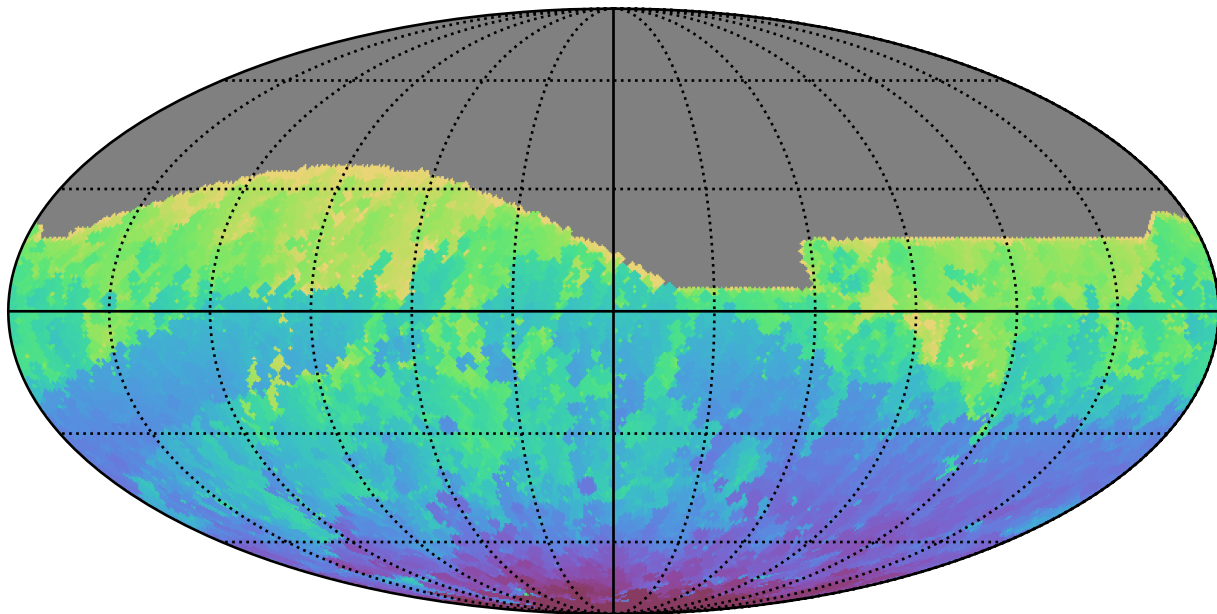
noroll_mjdp60_v3.4_10yrs All sky i band: Min HA
