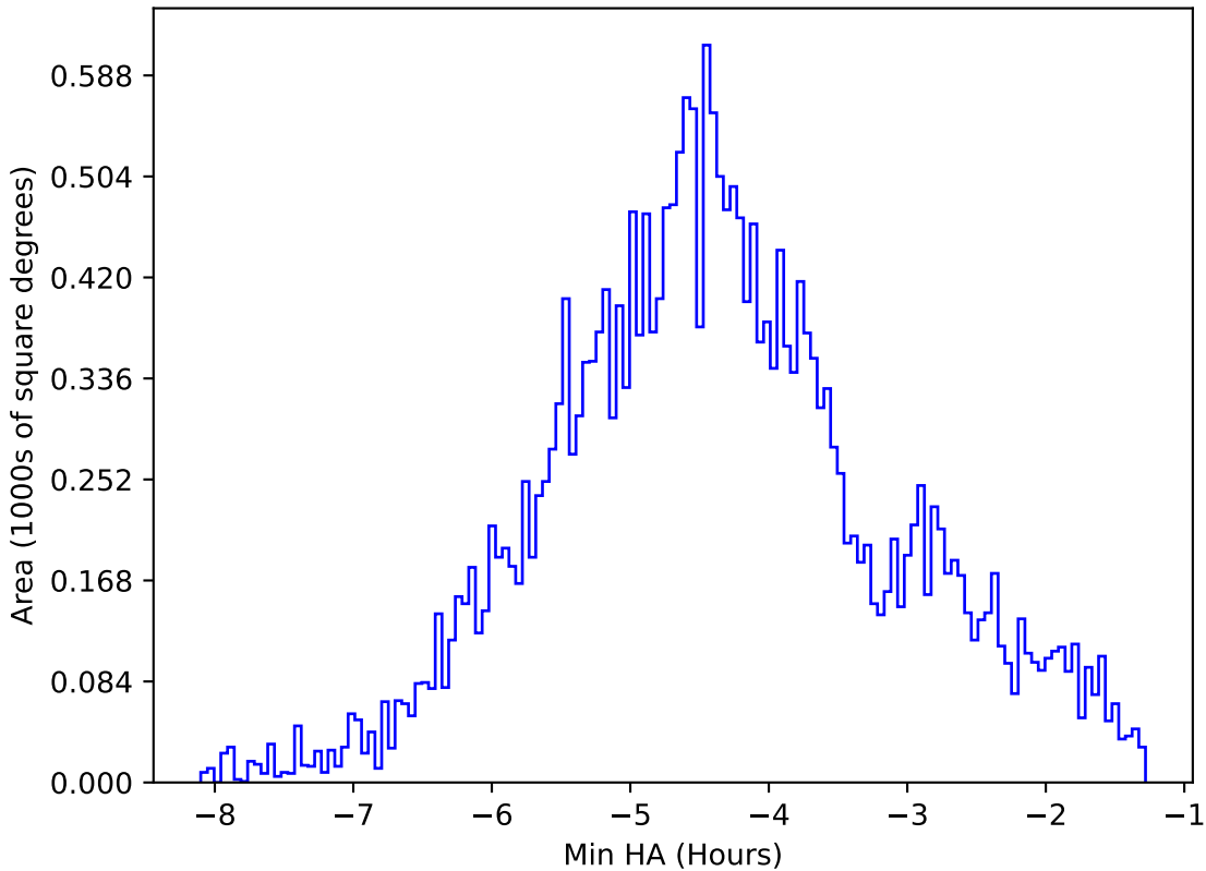
noroll_mjdp60_v3.4_10yrs All sky all bands: Min HA
