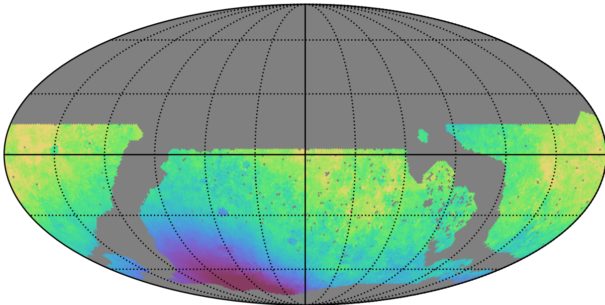
noroll_mjdp60_v3.4_10yrs WFD z band: Median solarElong
