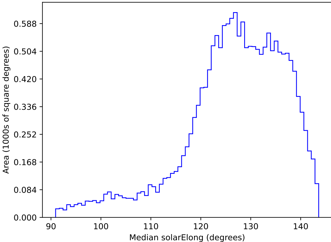
noroll_mjdp60_v3.4_10yrs WFD z band: Median solarElong
