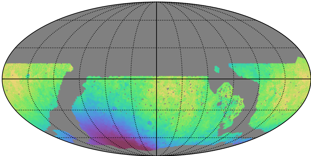
noroll_mjdp60_v3.4_10yrs WFD y band: Median solarElong
