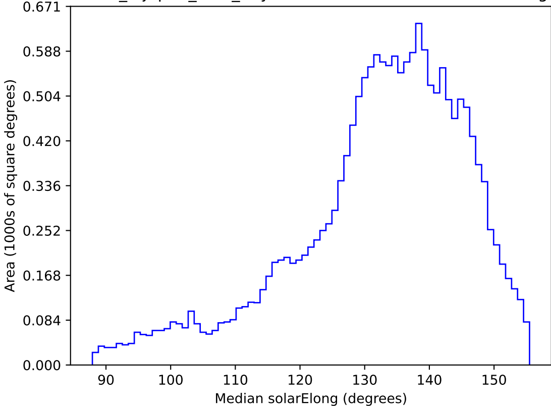
noroll_mjdp60_v3.4_10yrs WFD u band: Median solarElong
