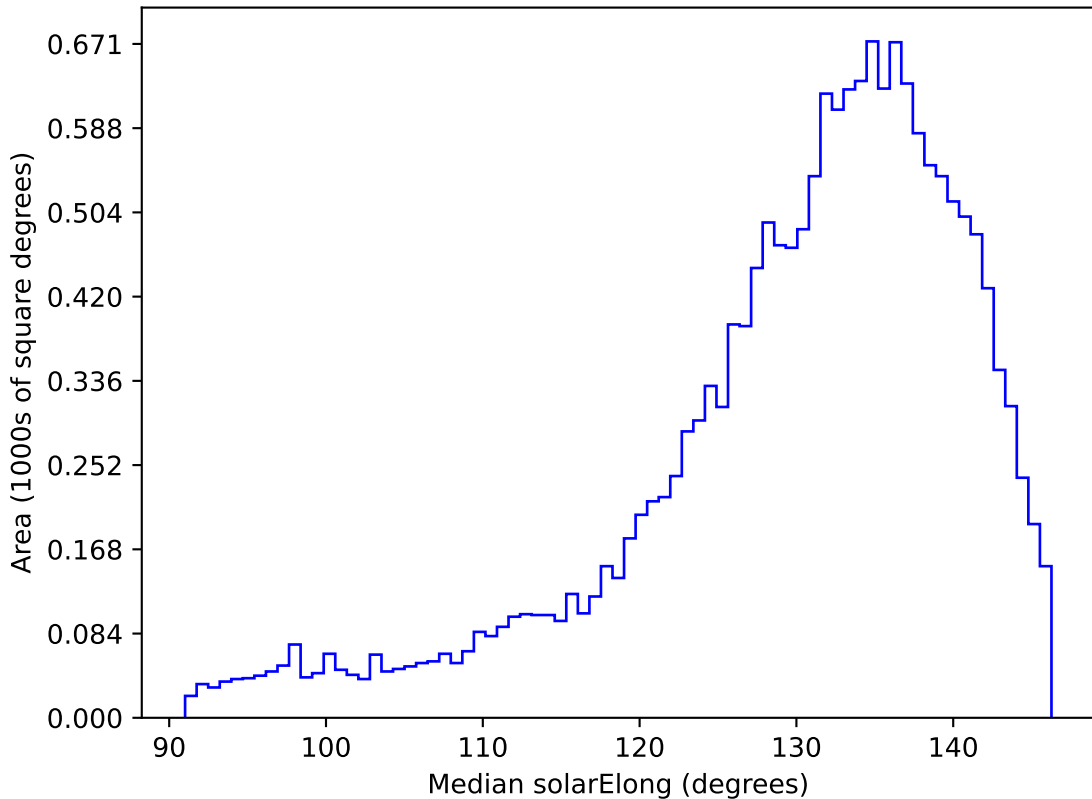
noroll_mjdp60_v3.4_10yrs WFD r band: Median solarElong
