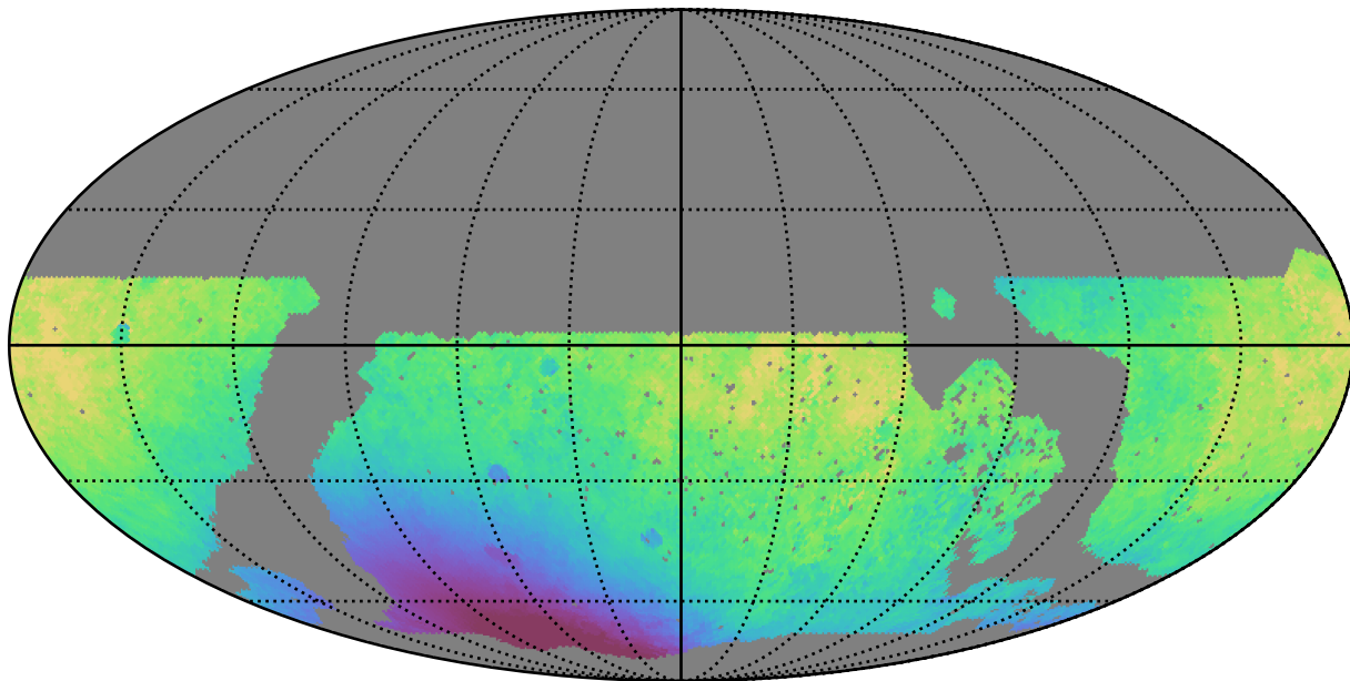
noroll_mjdp60_v3.4_10yrs WFD i band: Median solarElong
