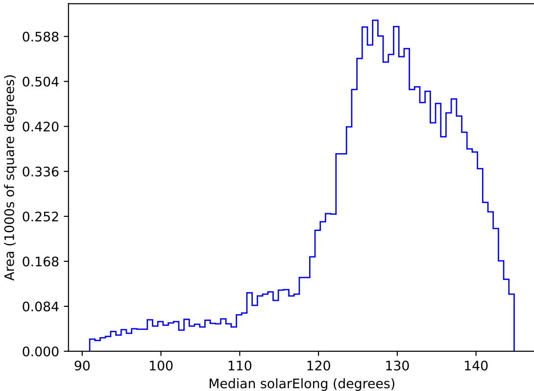
noroll_mjdp60_v3.4_10yrs WFD i band: Median solarElong
