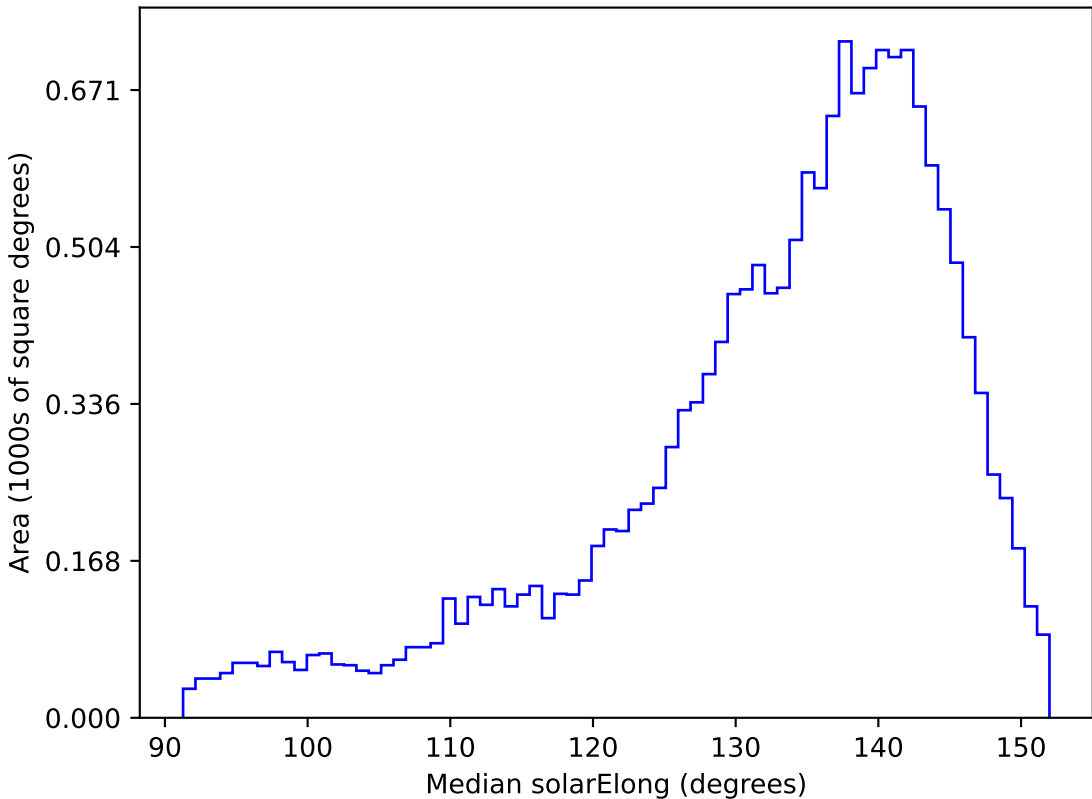
noroll_mjdp60_v3.4_10yrs WFD g band: Median solarElong
