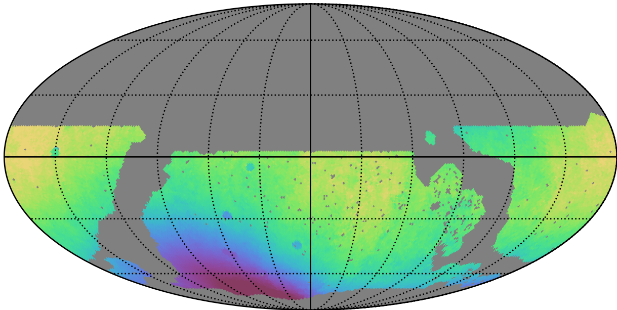
noroll_mjdp60_v3.4_10yrs WFD all bands: Median solarElong
