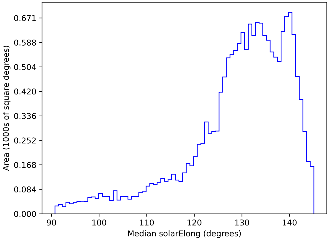
noroll_mjdp60_v3.4_10yrs WFD all bands: Median solarElong
