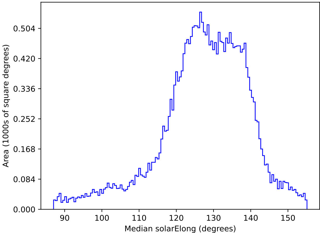
noroll_mjdp60_v3.4_10yrs All sky z band: Median solarElong
