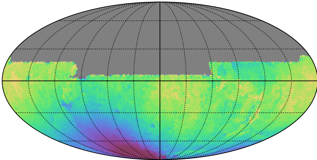
noroll_mjdp60_v3.4_10yrs All sky y band: Median solarElong
