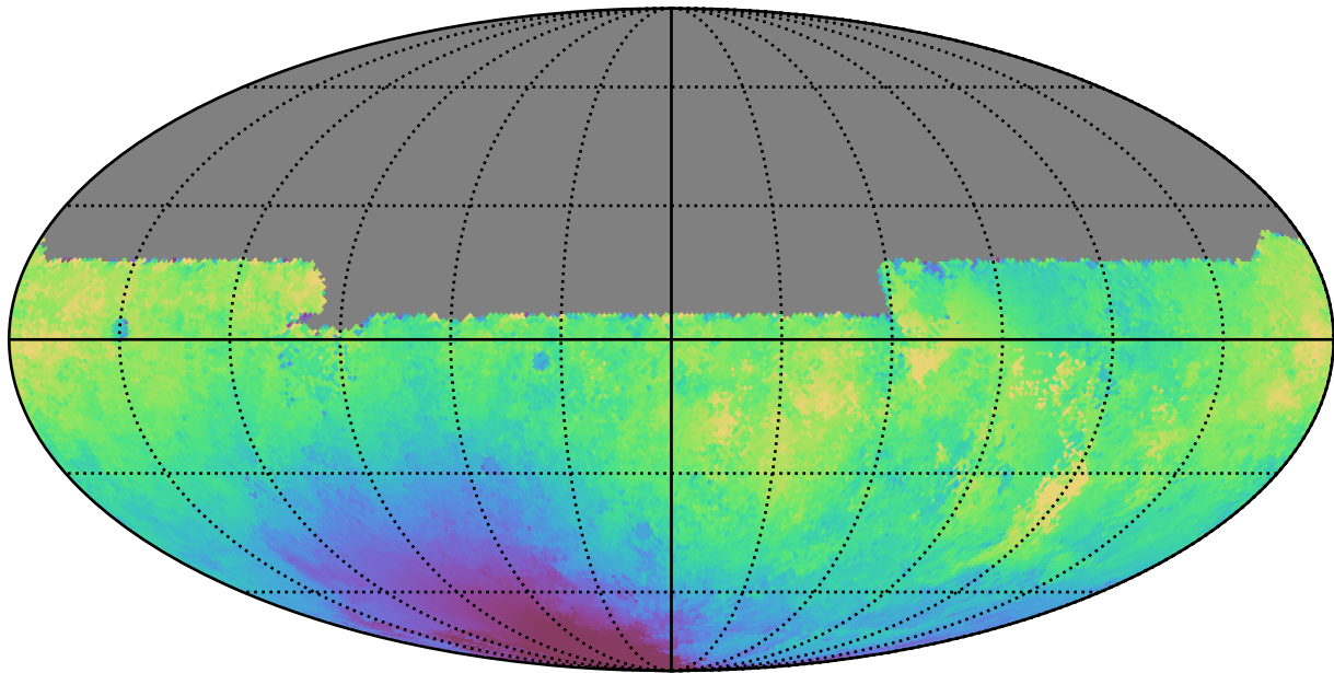
noroll_mjdp60_v3.4_10yrs All sky u band: Median solarElong
