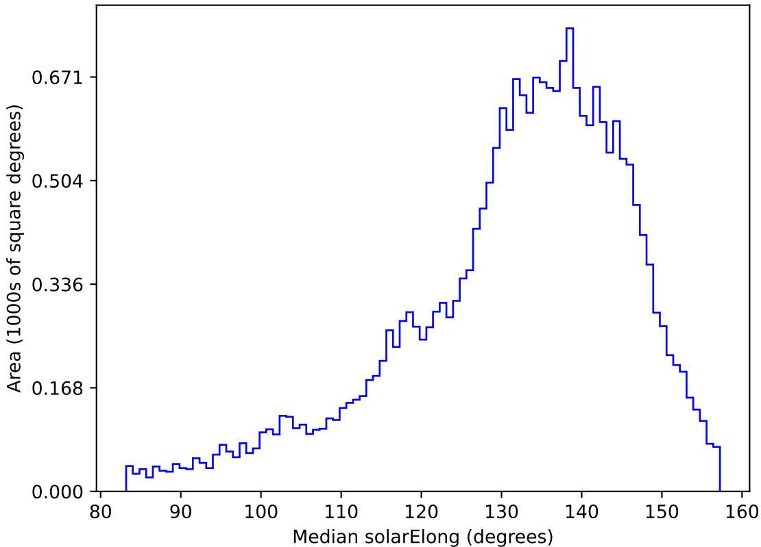
noroll_mjdp60_v3.4_10yrs All sky u band: Median solarElong
