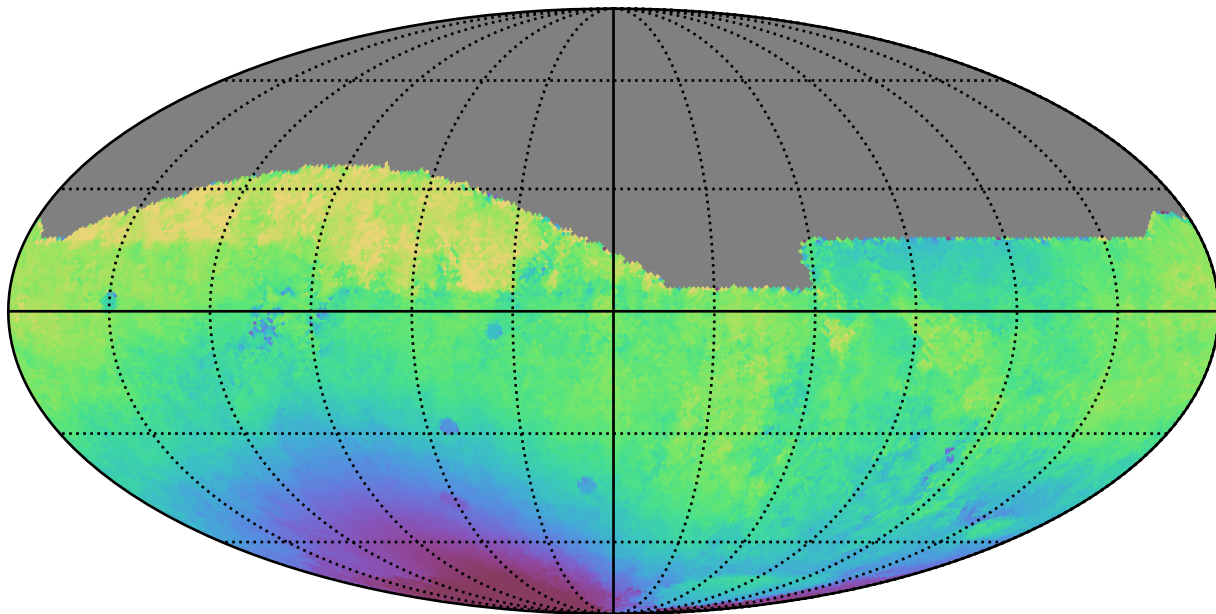
noroll_mjdp60_v3.4_10yrs All sky r band: Median solarElong
