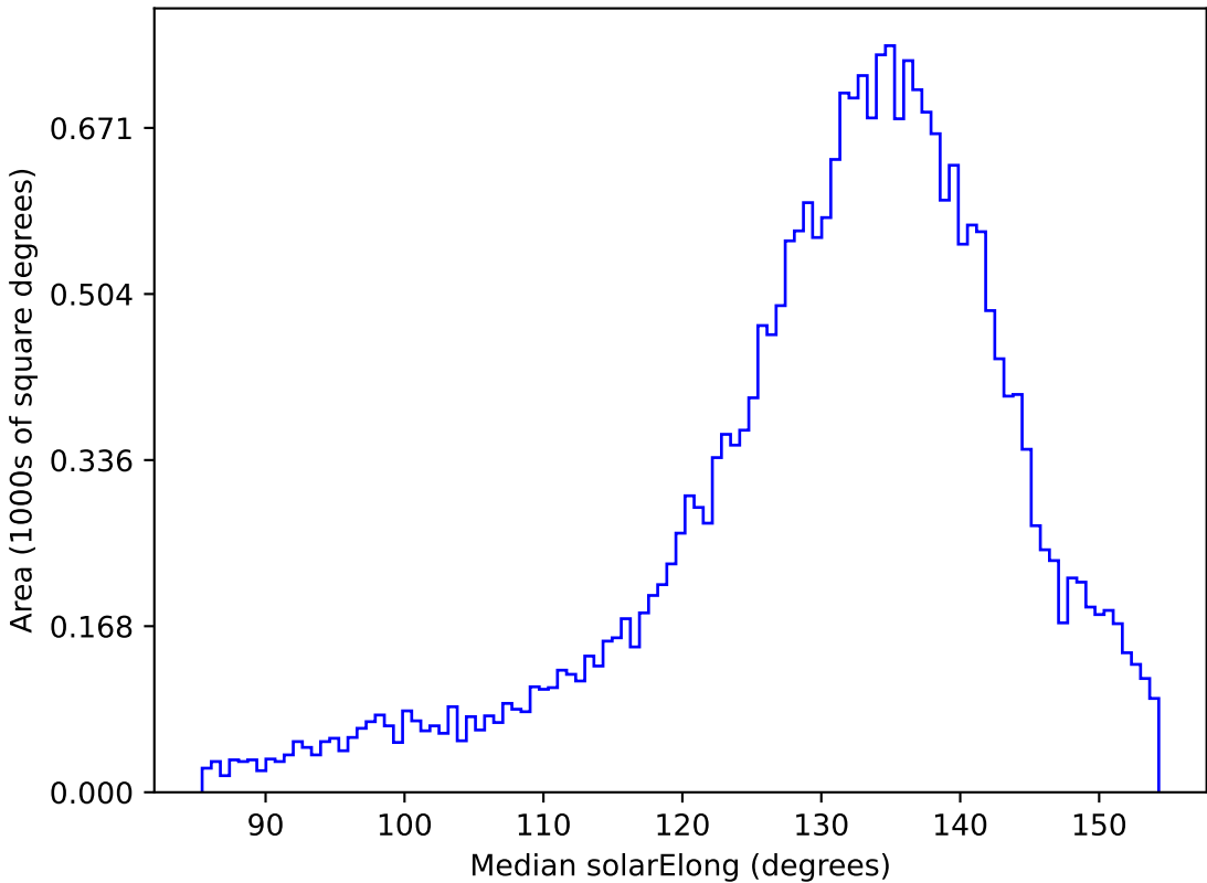
noroll_mjdp60_v3.4_10yrs All sky r band: Median solarElong
