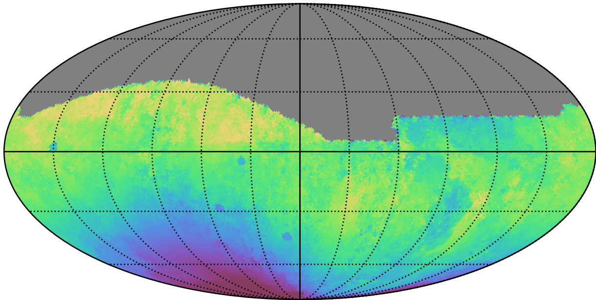
noroll_mjdp60_v3.4_10yrs All sky g band: Median solarElong
