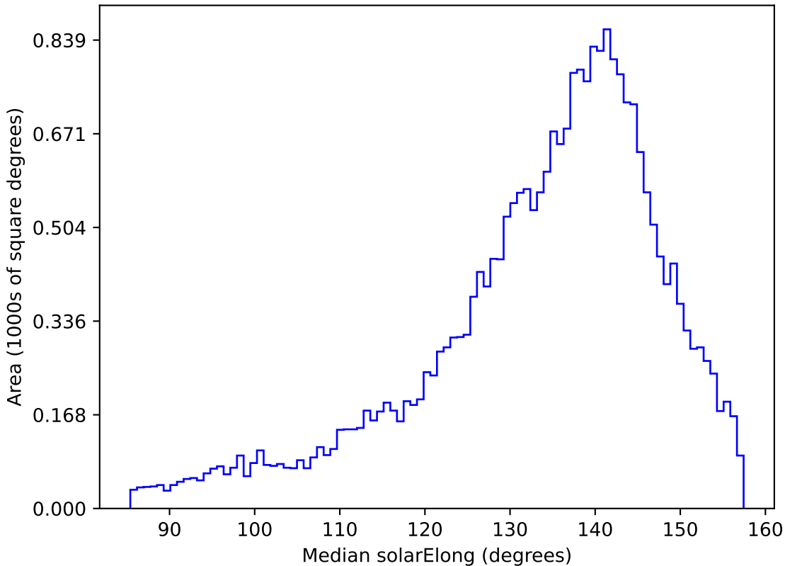
noroll_mjdp60_v3.4_10yrs All sky g band: Median solarElong
