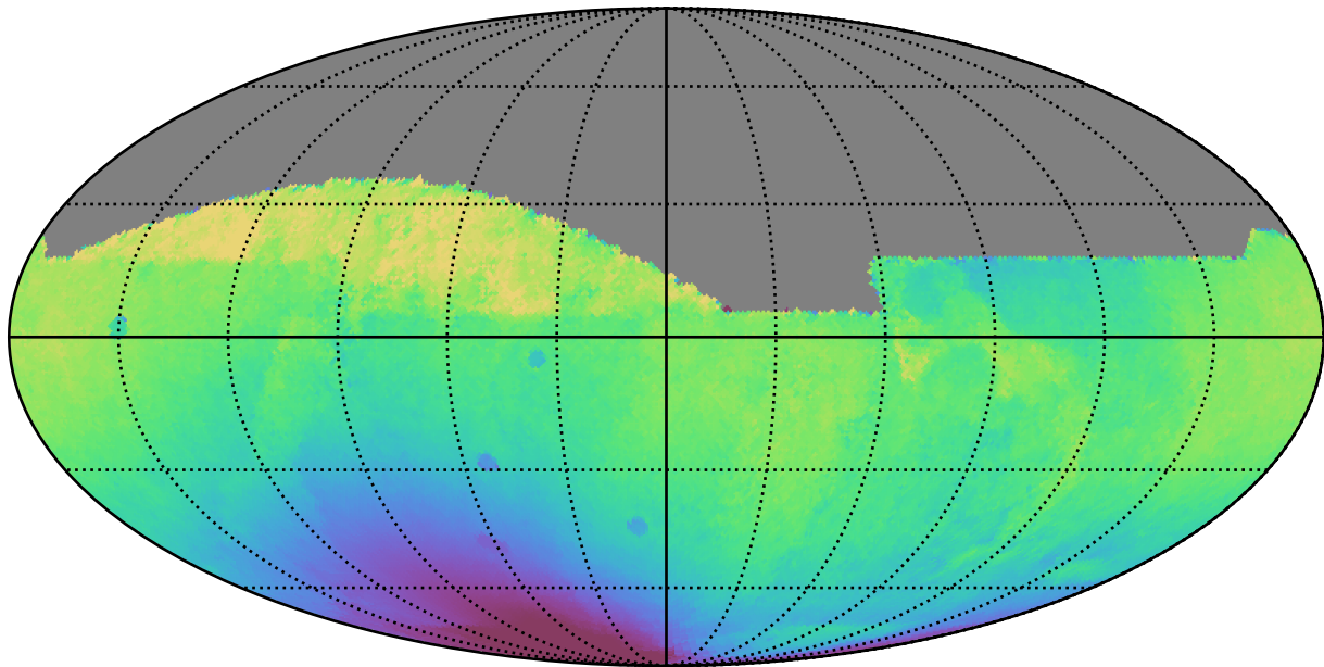
noroll_mjdp60_v3.4_10yrs All sky all bands: Median solarElong
