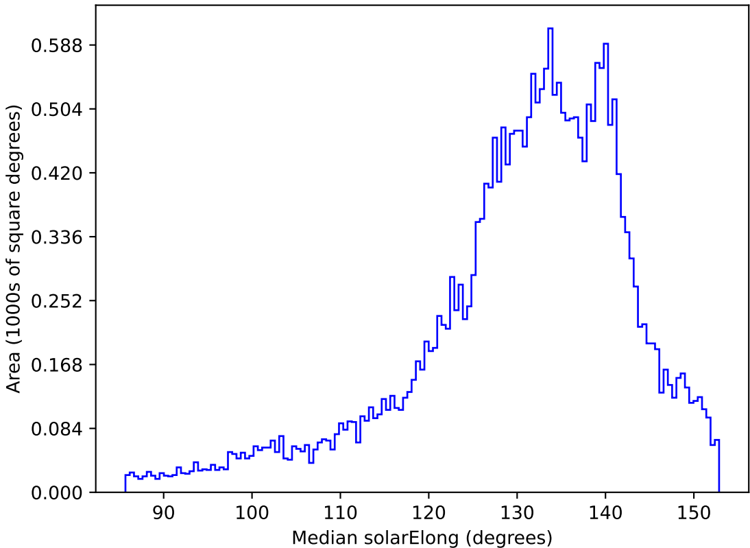
noroll_mjdp60_v3.4_10yrs All sky all bands: Median solarElong
