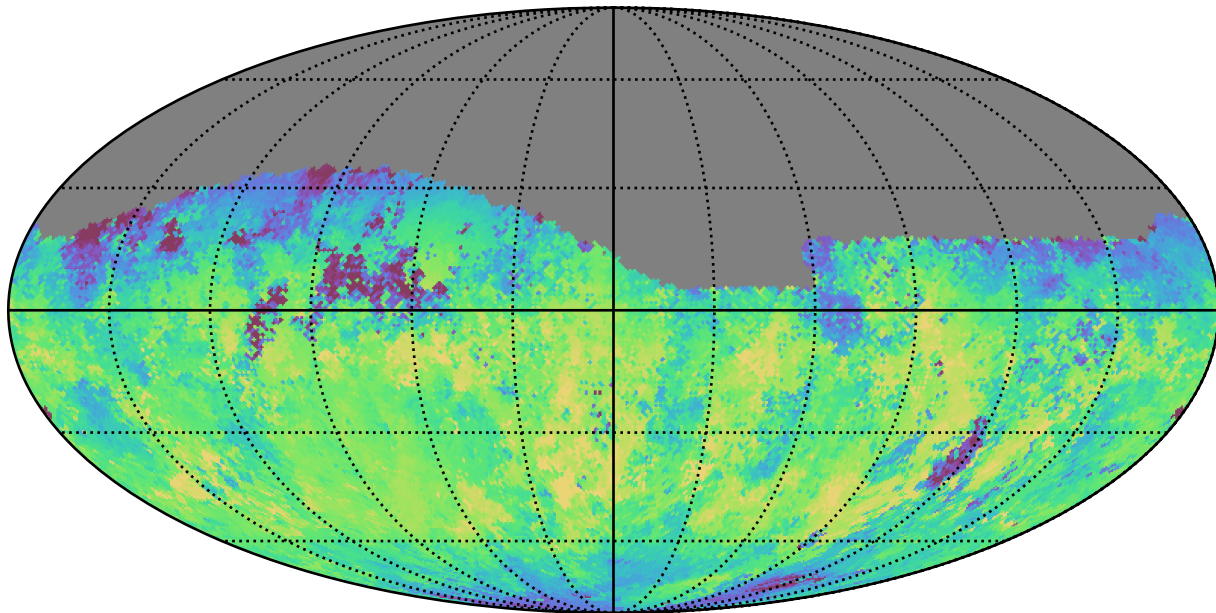
noroll_mjdp60_v3.4_10yrs Yr 1 z band: Median skyBrightness
