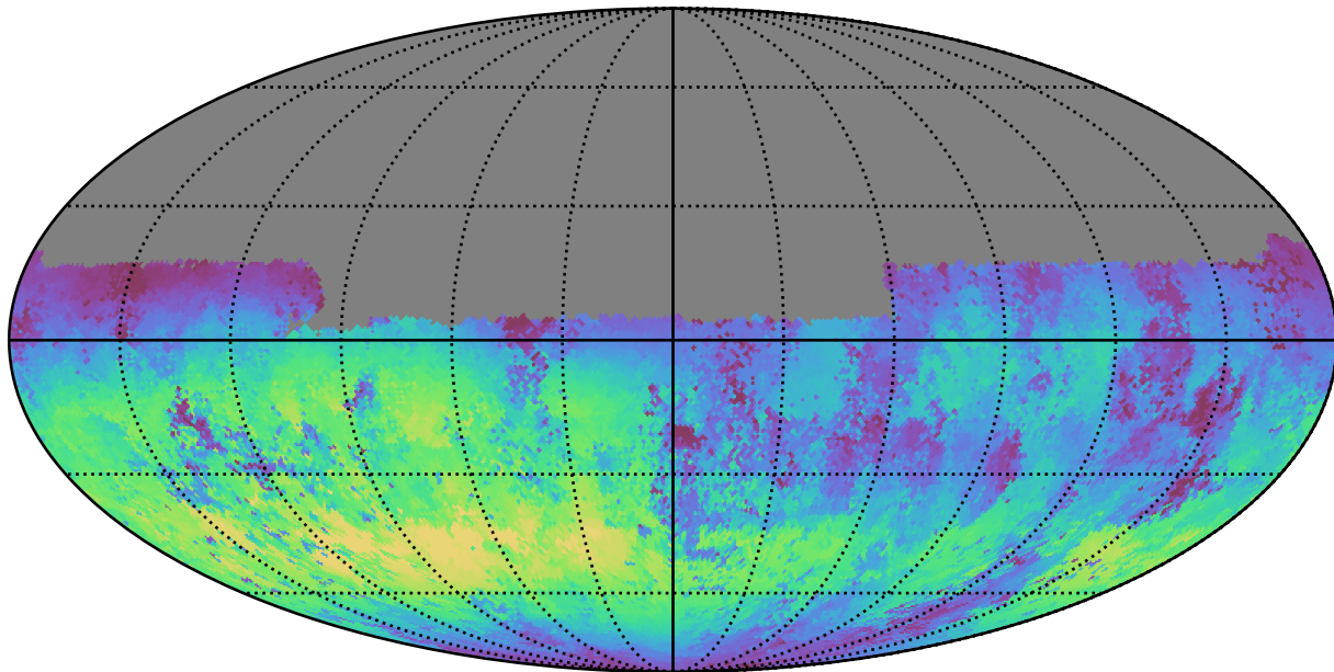
noroll_mjdp60_v3.4_10yrs Yr 1 u band: Median skyBrightness
