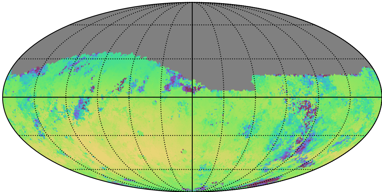
noroll_mjdp60_v3.4_10yrs Yr 1 r band: Median skyBrightness
