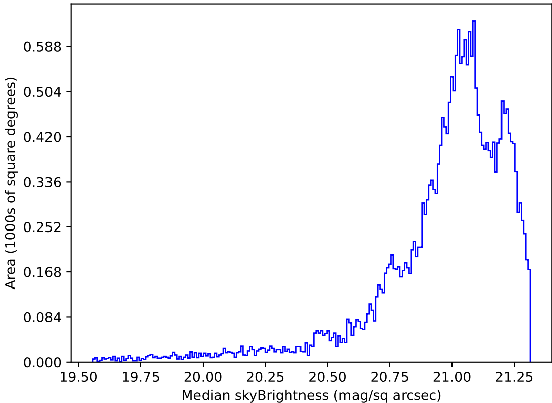
noroll_mjdp60_v3.4_10yrs Yr 1 r band: Median skyBrightness
