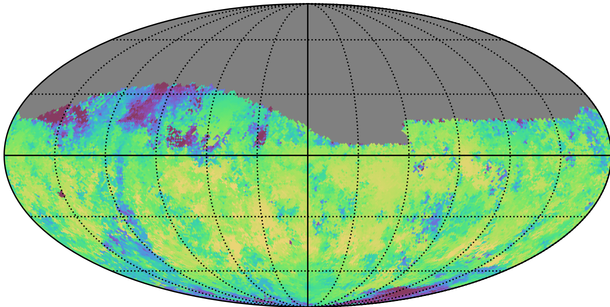
noroll_mjdp60_v3.4_10yrs Yr 1 i band: Median skyBrightness
