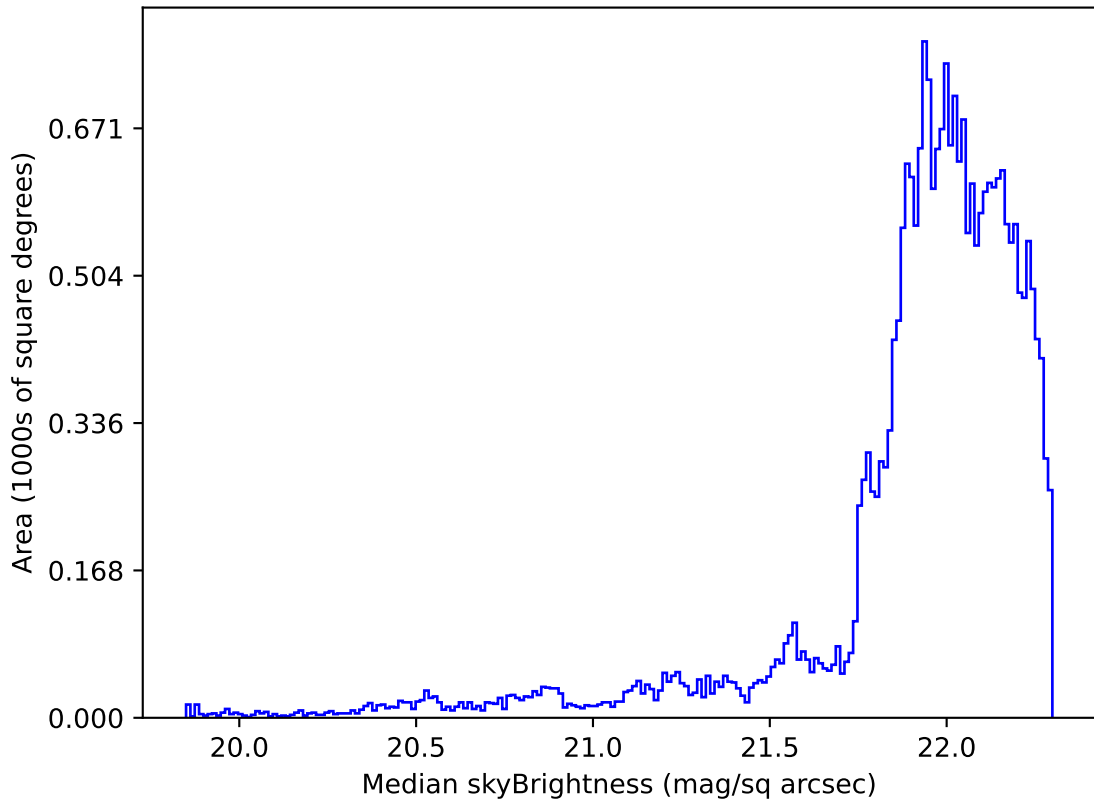
noroll_mjdp60_v3.4_10yrs Yr 1 g band: Median skyBrightness
