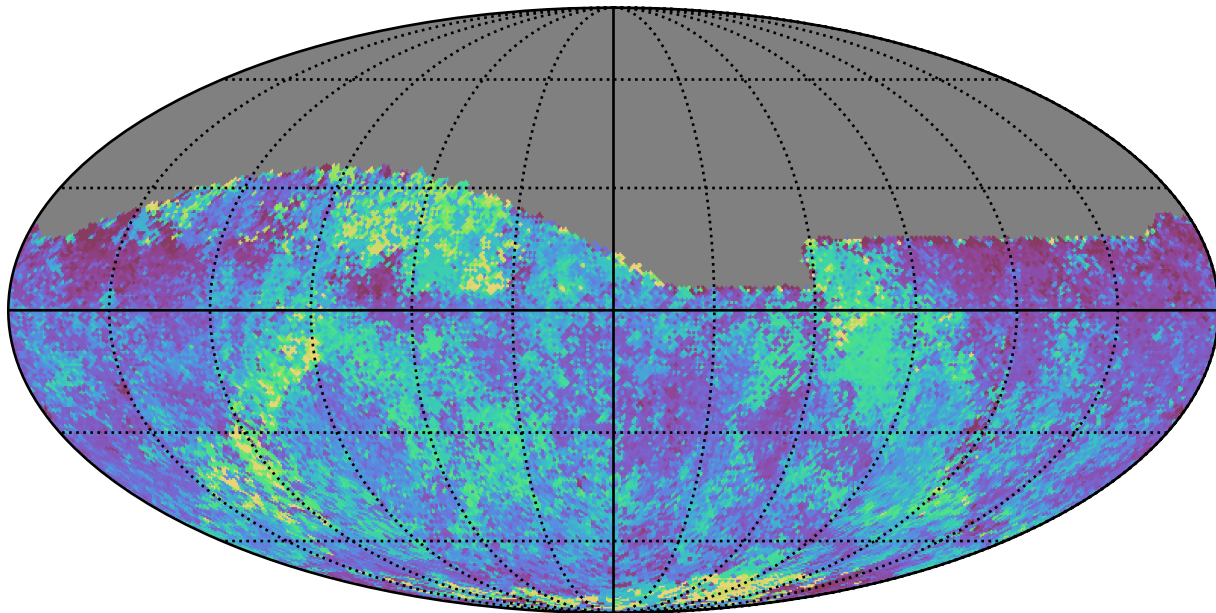
noroll_mjdp60_v3.4_10yrs Yr 1 all bands: Median skyBrightness
