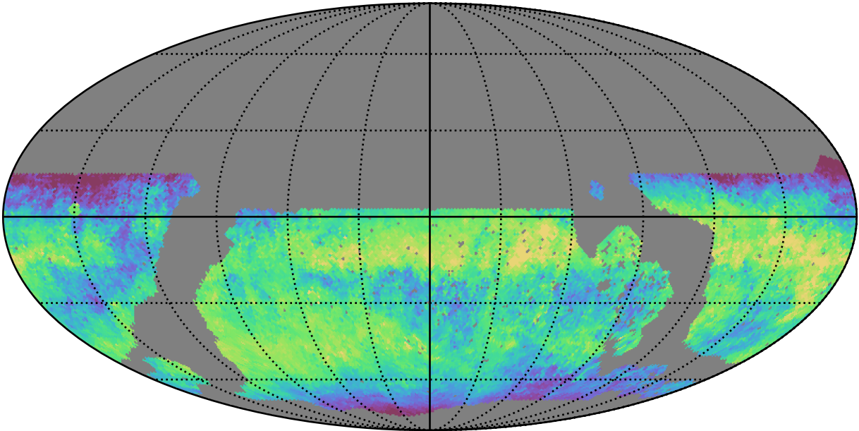
noroll_mjdp60_v3.4_10yrs WFD z band: Median skyBrightness
