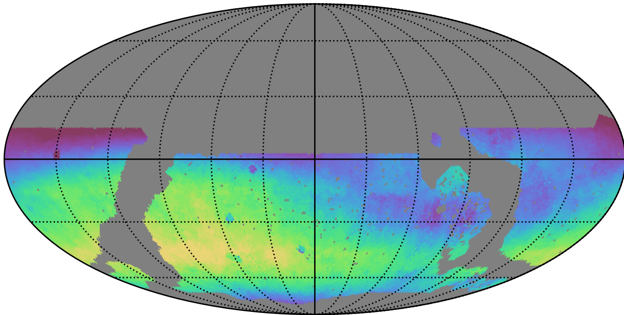
noroll_mjdp60_v3.4_10yrs WFD u band: Median skyBrightness
