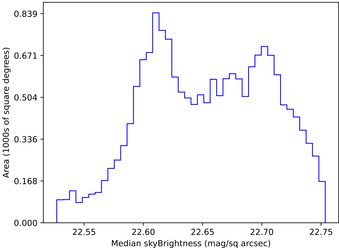
noroll_mjdp60_v3.4_10yrs WFD u band: Median skyBrightness
