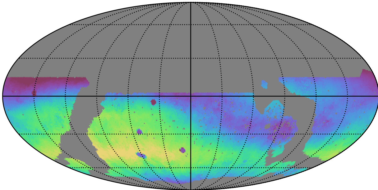
noroll_mjdp60_v3.4_10yrs WFD r band: Median skyBrightness
