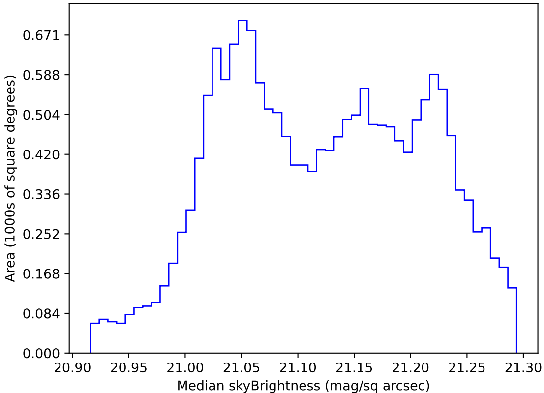
noroll_mjdp60_v3.4_10yrs WFD r band: Median skyBrightness
