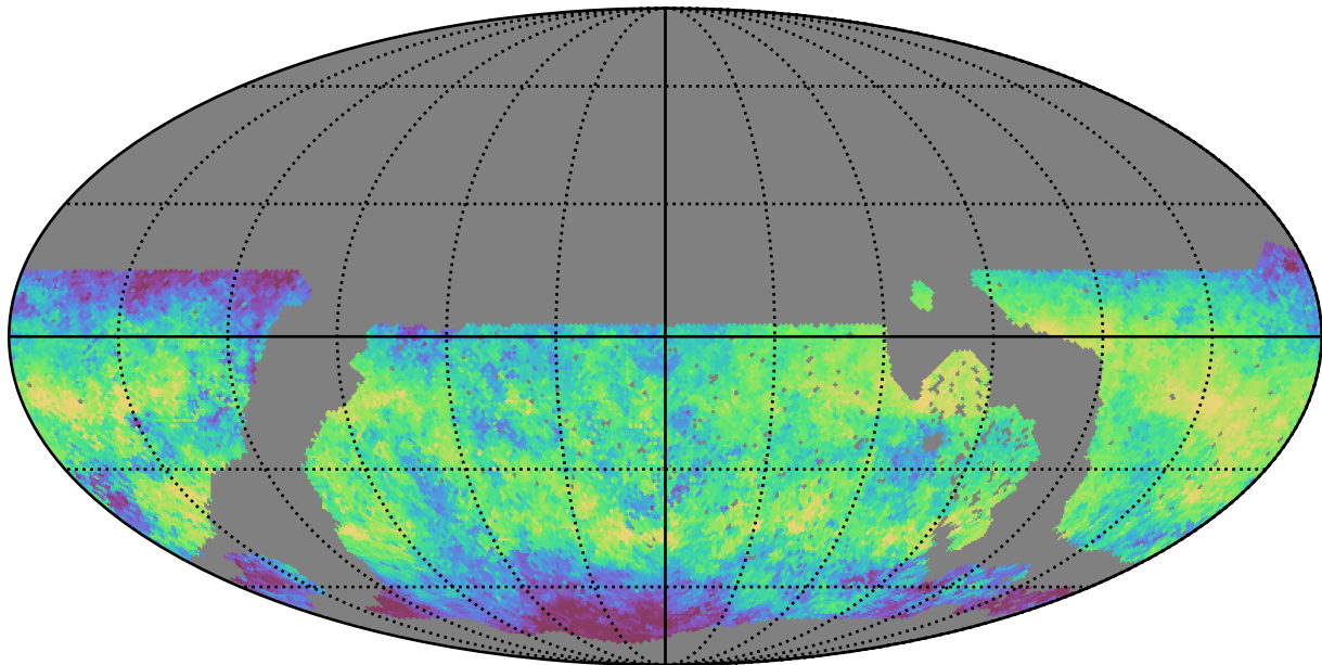
noroll_mjdp60_v3.4_10yrs WFD i band: Median skyBrightness
