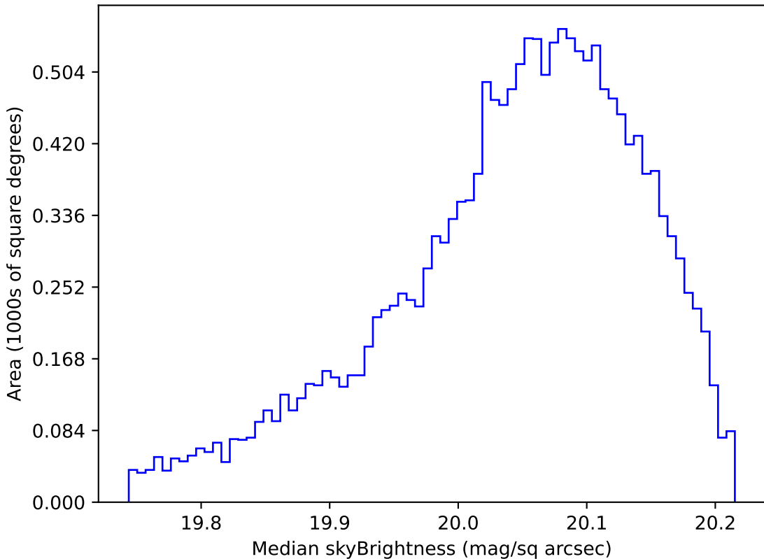
noroll_mjdp60_v3.4_10yrs WFD i band: Median skyBrightness
