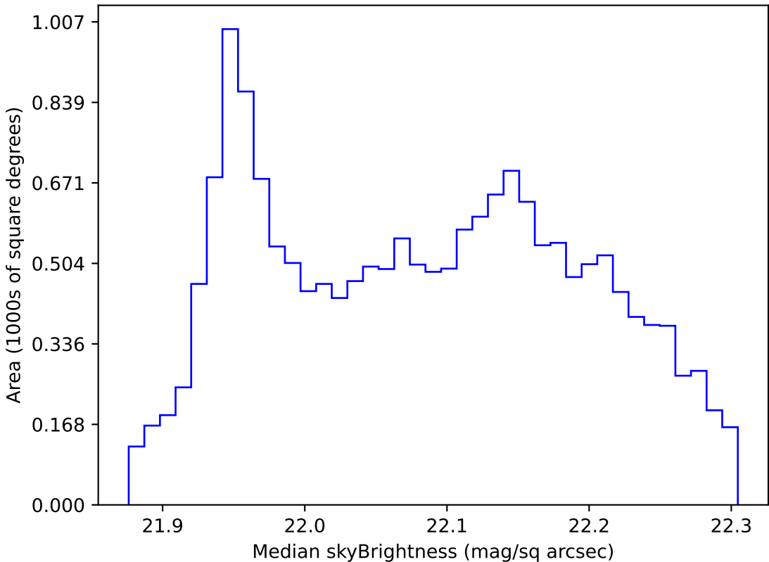
noroll_mjdp60_v3.4_10yrs WFD g band: Median skyBrightness
