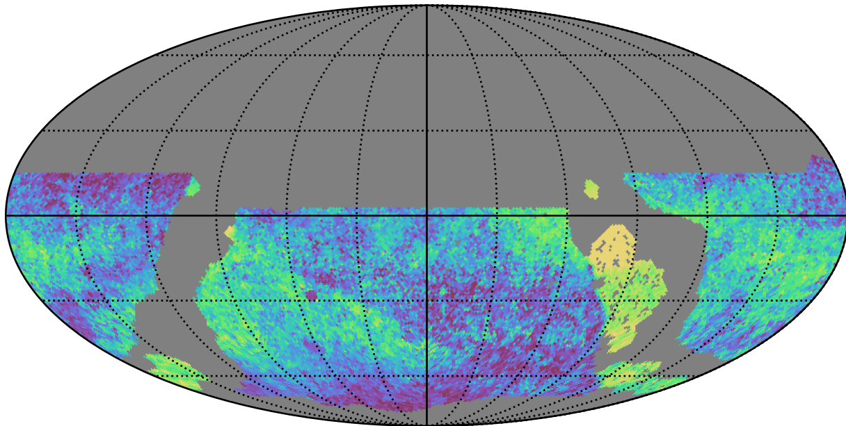
noroll_mjdp60_v3.4_10yrs WFD all bands: Median skyBrightness
